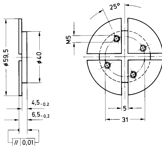
Fig. 8.2: Mounting plate
