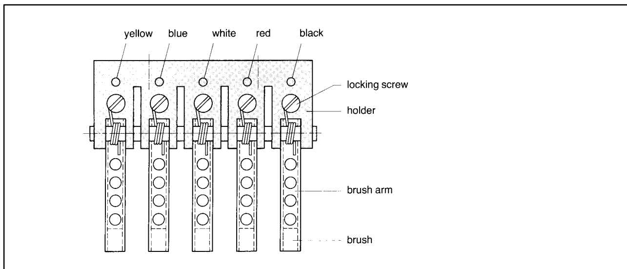
Fig. 9.2: Brush holder SK5/ZB
