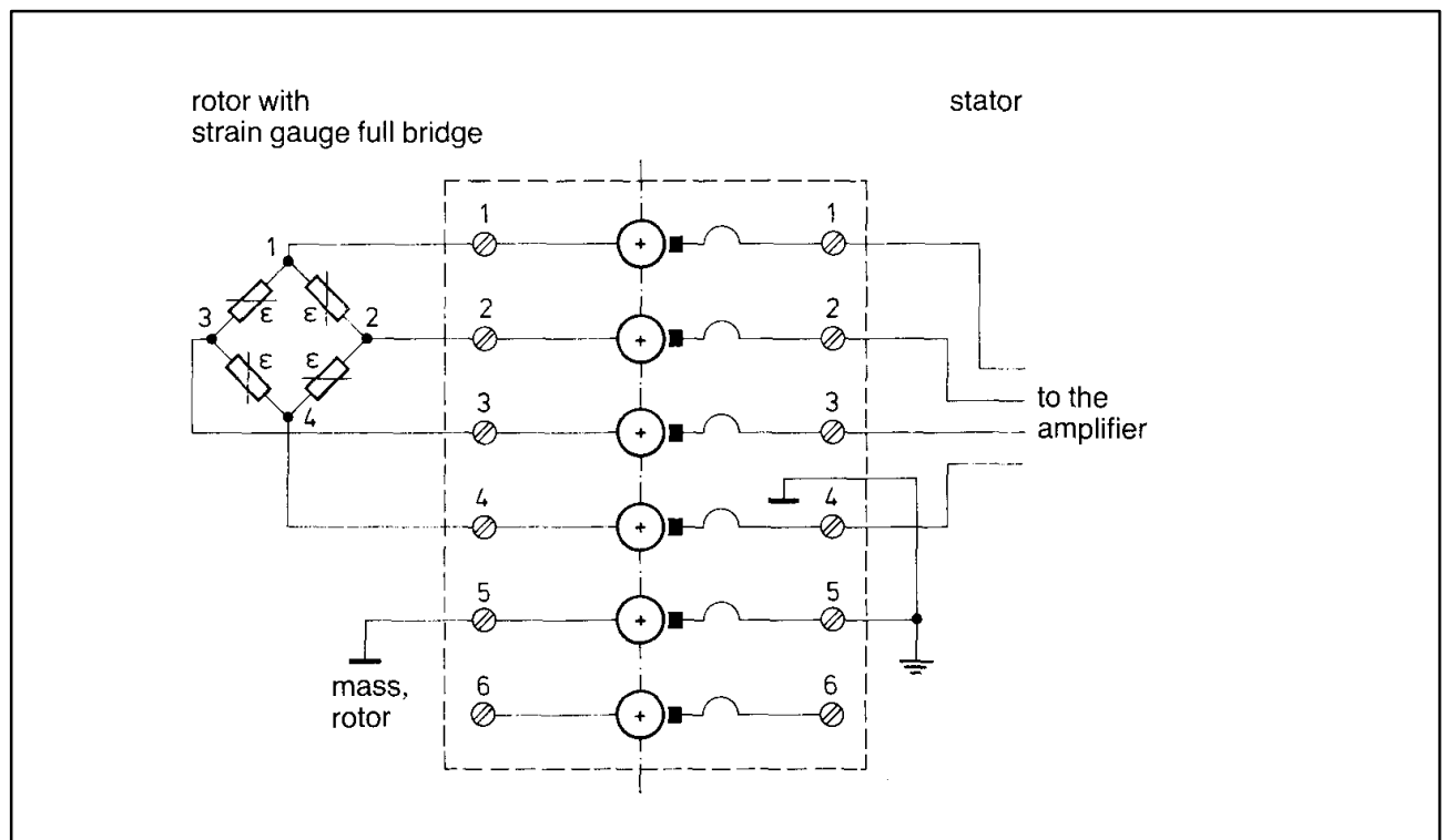
Abb. 5.1: Mounting without mounting plate
